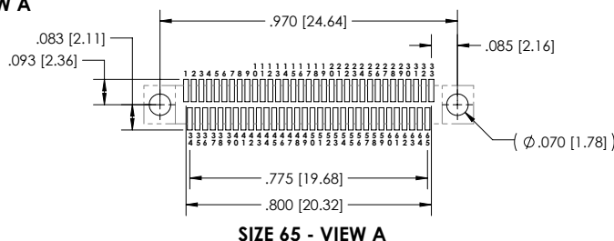
SIZE 65 - VIEW A
