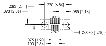
SIZE 9 - VIEW A
