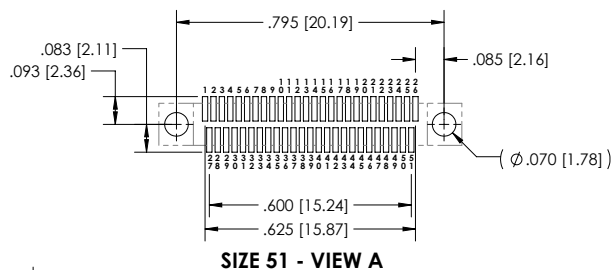
SIZE 51 - VIEW A
