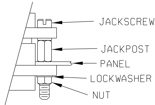
REAR PANEL MOUNT (CONSULT FACTORY)
