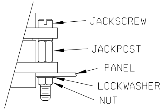
FRONT PANEL MOUNT
